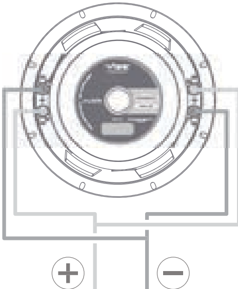
Parallel 1\Omega Impedance
